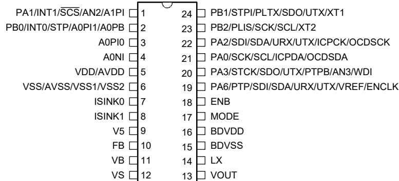
BA45F25343/BA45V25343 24 SSOP-A
