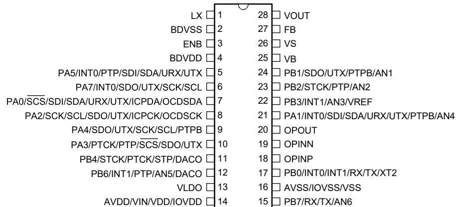
BA45F6850/BA45V6850 28 SOP-A
