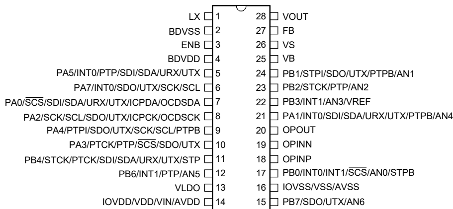
BA45F6840/BA45V6840 28 SSOP-A
