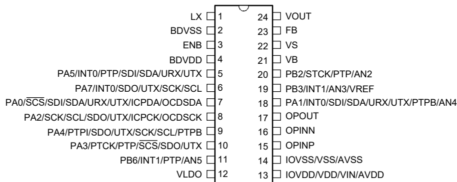
BA45F6840/BA45V6840 24 SSOP-A
