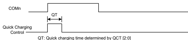
R 型偏压配置 - 1/3 Bias
