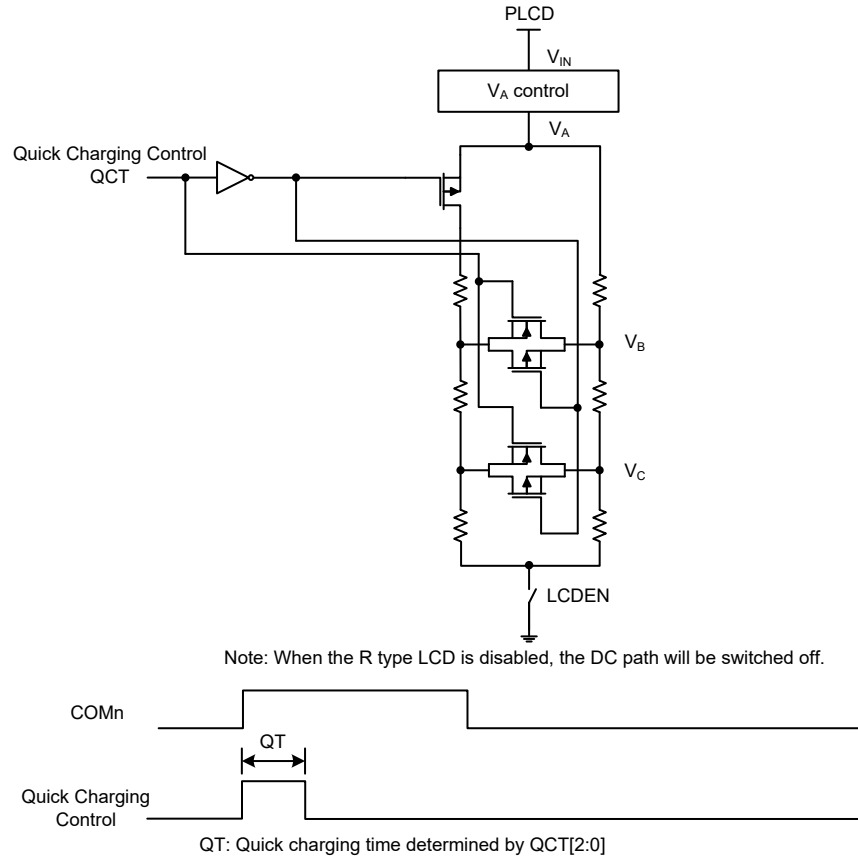
R 型偏压配置 – 1/3 Bias
