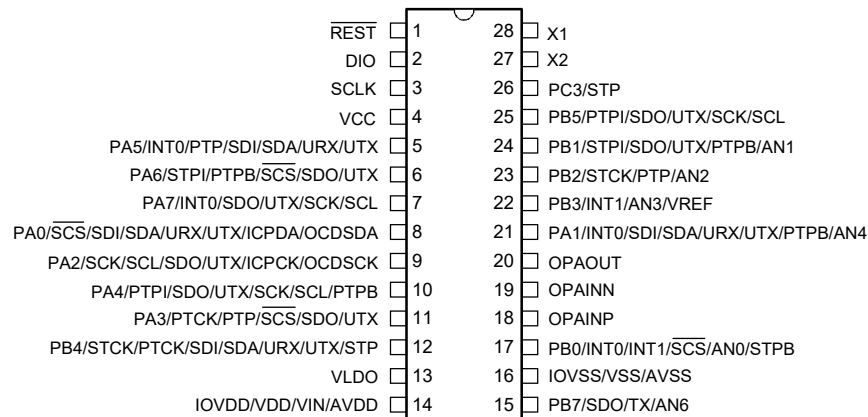
BA45F6742/BA45V6742 28 SSOP-A
