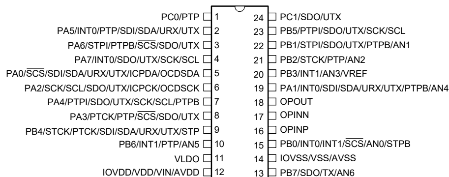
BA45F6740/BA45V6740 24 SSOP-A
