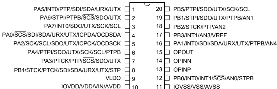
BA45F6740/BA45V6740 20 SSOP-A
