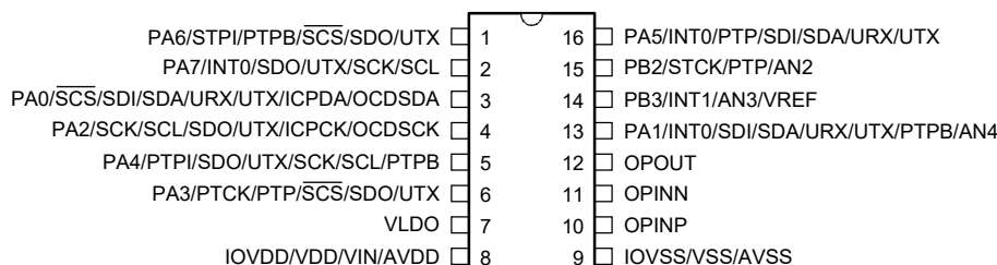
BA45F6740/BA45V6740 16 NSOP-A
