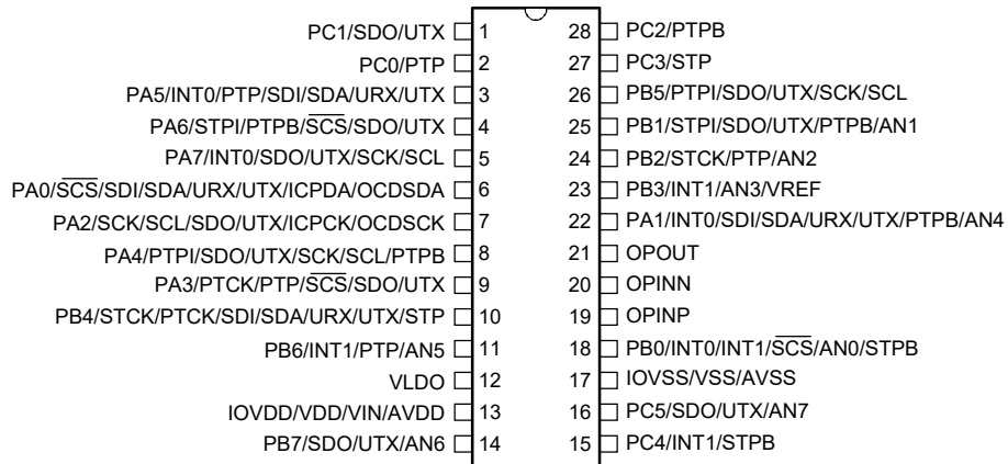
BA45F6740/BA45V6740 28 SSOP-A
