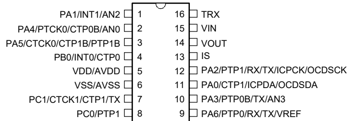
BA45F5541/BA45V5541 16 NSOP-A
