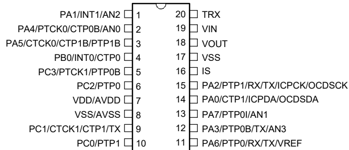
BA45F5541/BA45V5541 20 SSOP-A
