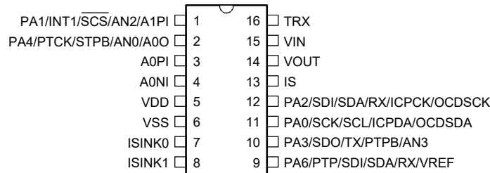
BA45F5542/BA45V5542 16 NSOP-A
