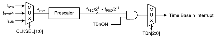
时基中断 ( n=0 \sim 1 )
