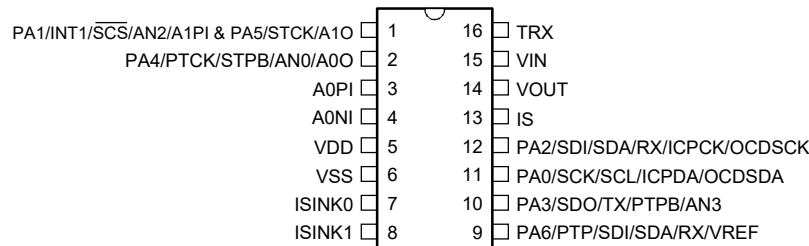
BA45F5542-2/BA45V5542-2 16 NSOP-A
