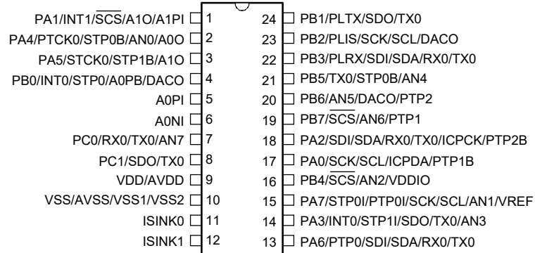
BA45F5260 24 SSOP-A
