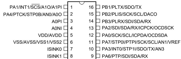
BA45F5250/BA45V5250 16 NSOP-A
