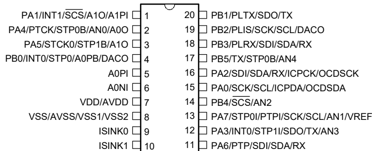
BA45F5250/BA45V5250 20 SSOP-A
